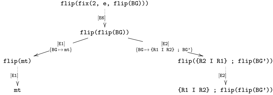
Figure 9: Folding variant narrowing tree for the goal \text{flip}(\text{fix}(2, e, \text{flip}(\text{BG}))) .
