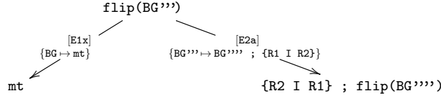
Figure 8: Folding variant narrowing tree for the goal \text{flip}(\text{BG}''') .
