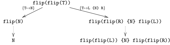
Figure 1: Folding variant narrowing tree for the goal \text{flip}(\text{flip}(T)) .
