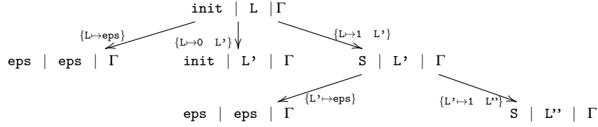
Figure 10: Folding variant narrowing tree for the goal \text{init} \mid L \mid \Gamma .
