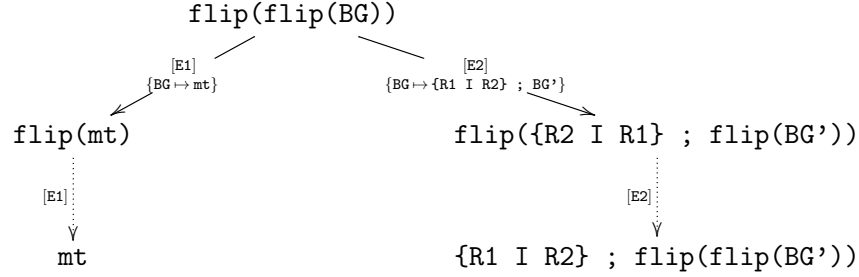
Figure 3: Folding variant narrowing tree for the goal \text{flip}(\text{flip}(\text{BG})) .
