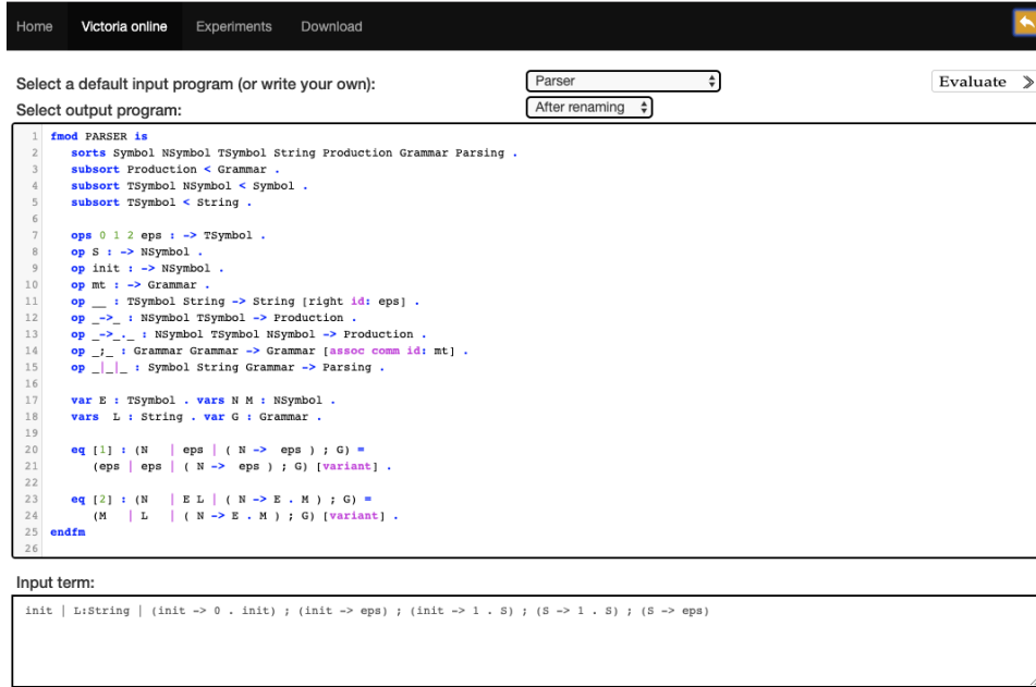
Figure 12: Specialization of the Parser example with Victoria
