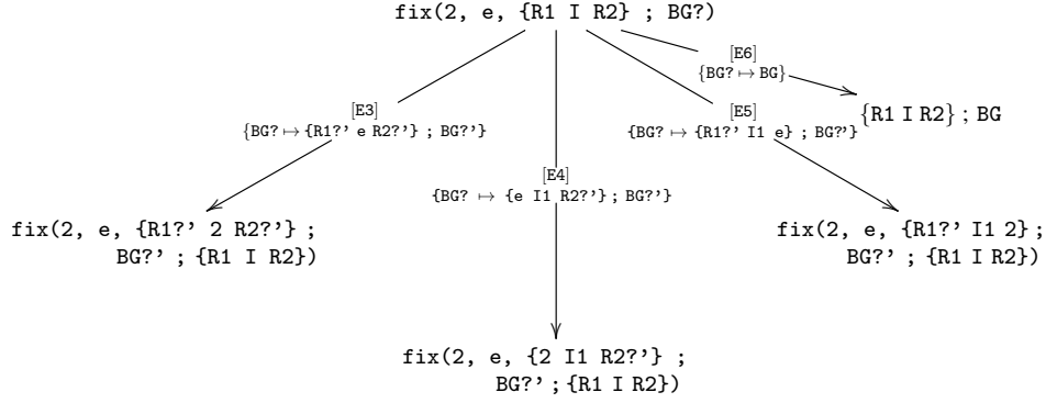
Figure 5: Folding variant narrowing tree for the goal \text{fix}(2, e, \{R1\ I\ R2\} ; BG?) .
