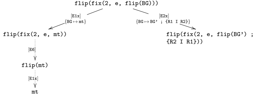
Figure 6: Folding variant narrowing tree for the goal \text{flip}(\text{fix}(2, e, \text{flip}(\text{BG}))) .
