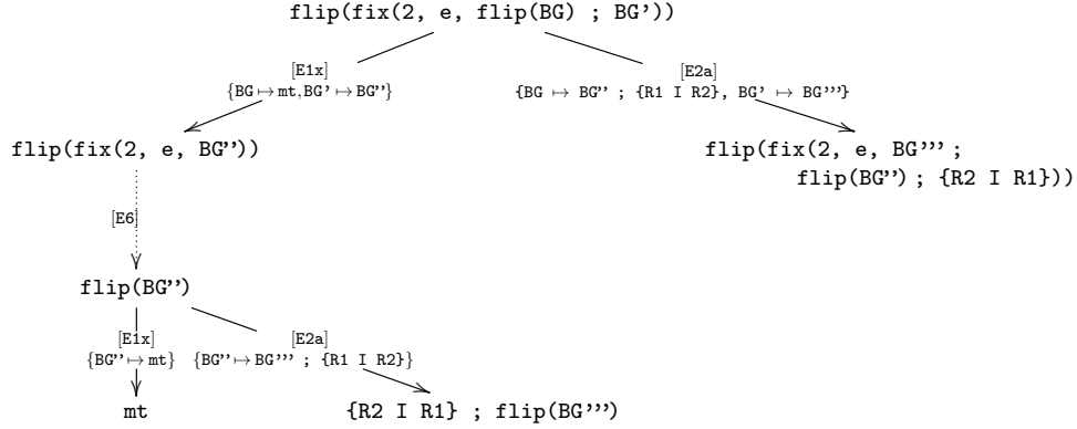
Figure 7: Folding variant narrowing tree for the goal \text{flip}(\text{fix}(2, e, \text{flip}(\text{BG}) ; \text{BG}')) .
