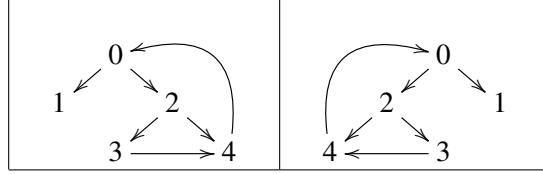
Figure 2: A binary graph (left) and its flipped version (right).
